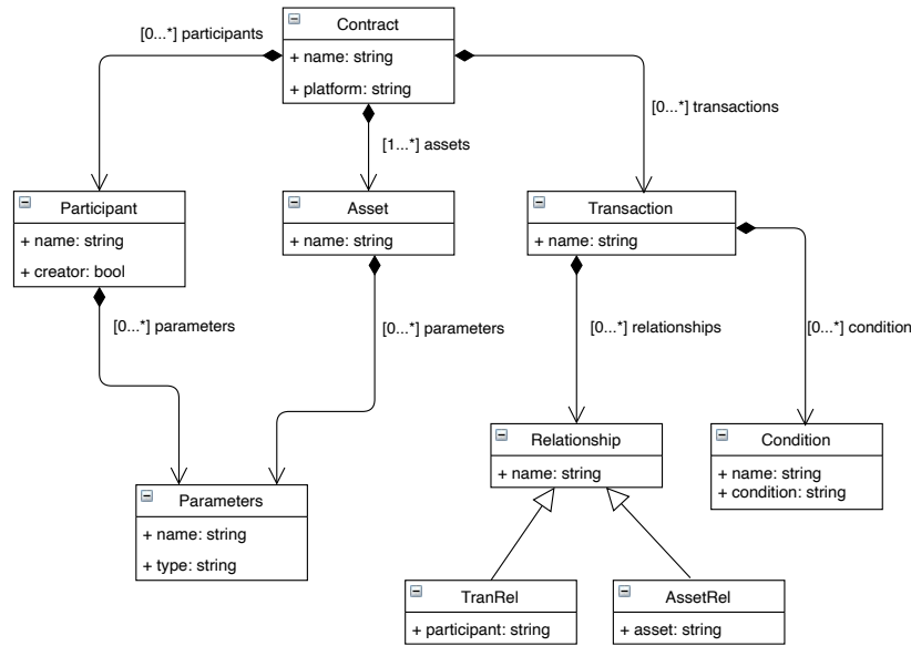
Fig. 3. Intention DSL
