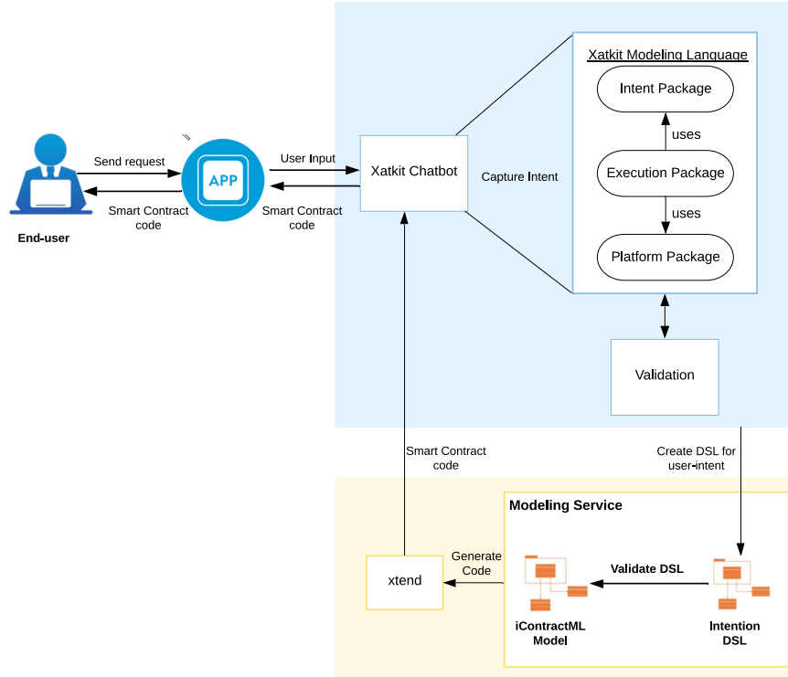
Fig. 1. iContractBot system architecture
